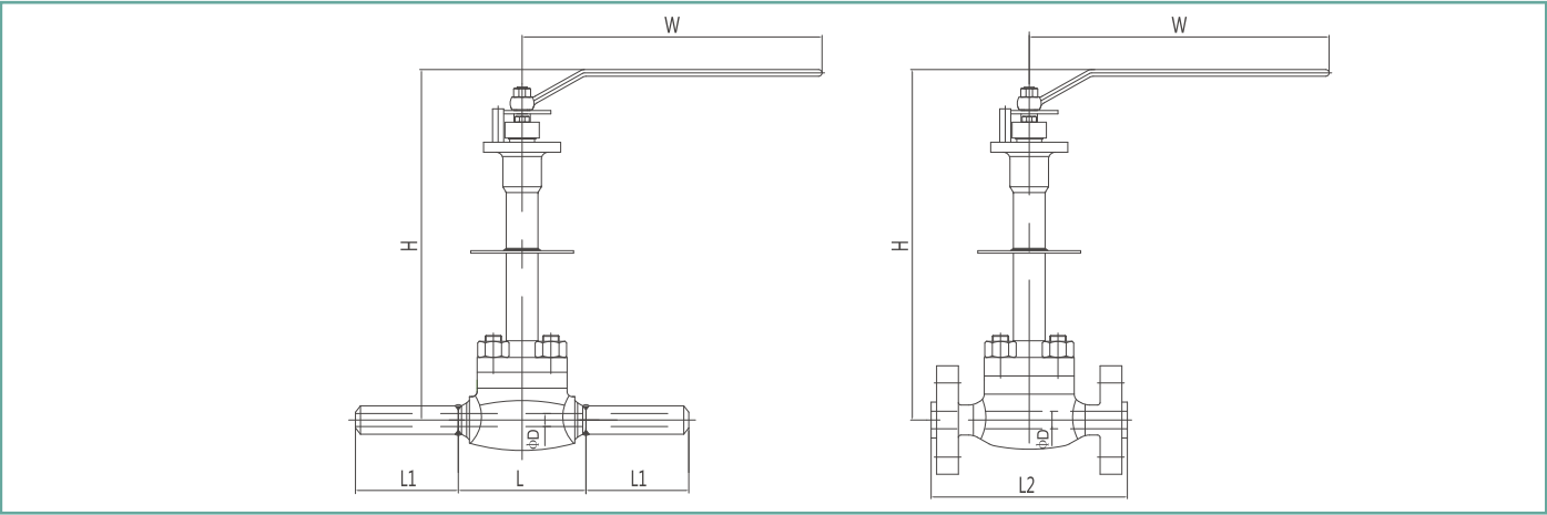
Class 150 / 300 / 600
